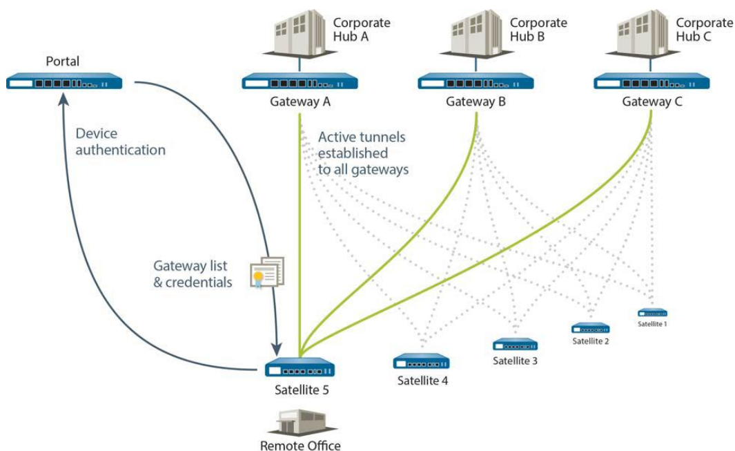
Figure 3-27: The GlobalProtect LSVPN components work together to securely extend an enterprise network to remote offices
