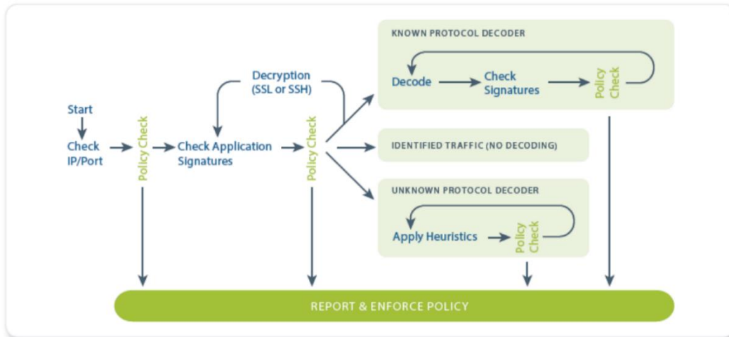
Figure 3-4: How Palo Alto Networks App-ID classifies applications
