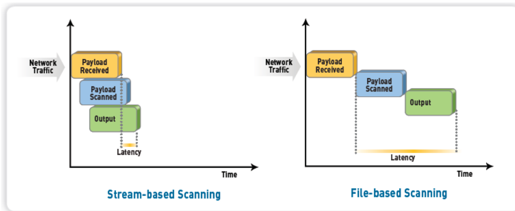
Figure 3-7: Stream-based scanning helps minimize latency and maximize throughput performance
